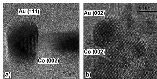
Figure 3. HREM images of: a) gold-tipped nanorods, with the (111) gold lattice planes parallel to the (002) of the cobalt nanorod (relaxed growth) and b) gold-decorated nanorod, in which the Au particles grow epitaxially on the nanorod sides, and the (002) gold lattice planes are aligned with the (002) of the cobalt.
