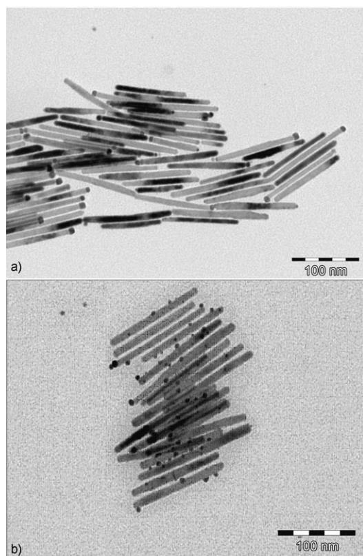
Figure 2. TEM images of a) gold-tipped Co nanorods prepared at 40°C and b) gold-decorated Co nanorods prepared at 20°C. For both, [\text{Co}] = 1.3 \times 10^{-3} \text{ M} , [\text{Au}] = 1.34 \times 10^{-4} \text{ M} , reaction time 48 h.
