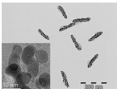
Figure 1. Gold formation around Co nanorods. Galvanic displacement almost completely destroys the Co structure. [\text{Co}] = 1.3 \times 10^{-3} \text{ M} , [\text{Au}] = 1.3 \times 10^{-4} \text{ M} , reaction time 30 min. Inset: HREM micrograph, in which only gold can be seen.
